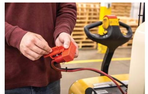
BatteryBlock™ Power Connector Lockout
